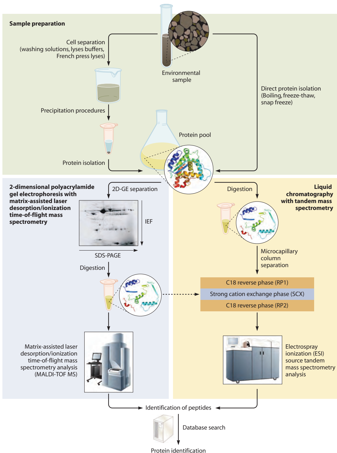
FIG. 1. Overview of two major environmental proteomic strategies. In one strategy (top left), proteins are separated by 2D-GE followed by MS analysis with either peptide mass mapping or LC-MS approaches. An alternate strategy (top right) involves protein digestion followed by online liquid LC separation and MS characterization. There are dramatic differences in measurement throughput, automation, and depth of protein identification for these two related but distinct approaches, as discussed in the text. IEF, isoelectric focusing; SDS, sodium dodecyl sulfate.
