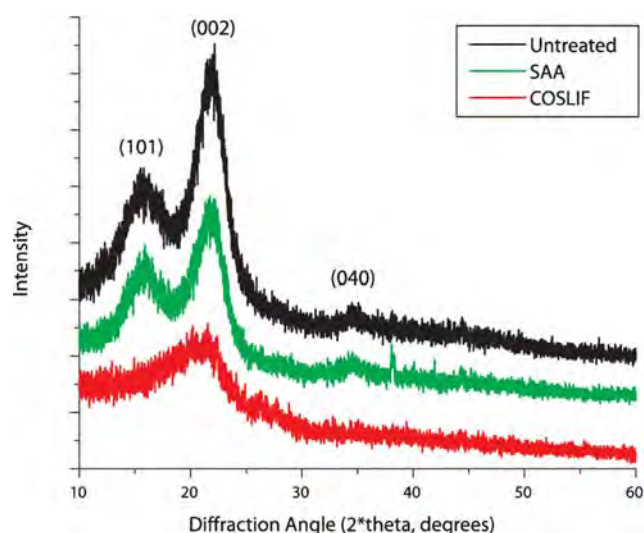
Figure 5. XRD diffraction spectra for untreated, COSLIF, and SAA switchgrass samples. The major peak seen for all three samples is the (0 0 2) peak, used for peak height-based CrI determination. (1 0 1) and (0 4 0) peaks are also apparent for untreated and SAA samples.
