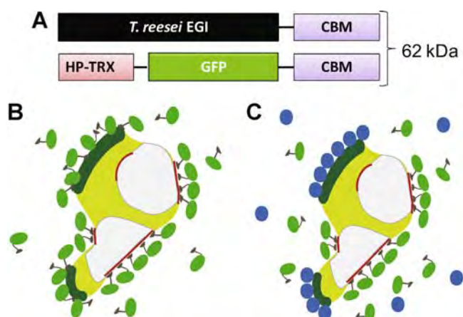
Figure 4. ThioRedoxin-GFP-CBM fusion protein schematic, with TGC proteins represented in green and BSA proteins in blue. The TGC protein is similar in size to T. reesei EGI (A). To determine total substrate accessibility to cellulase (TSAC), TGC equilibration is conducted without BSA (B). When BSA blocking is used prior to TGC equilibration, cellulose accessibility to cellulase (CAC) may be determined (C). Cellulose surfaces (110 face) susceptible to cellulase binding are highlighted in red.
