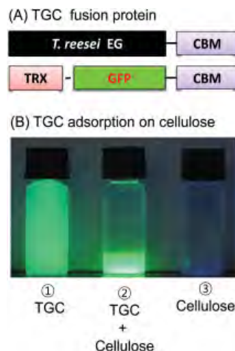
Figure 1. Schematic diagram of thioiodoxin-GFP-CBM fusion protein (A). The TGC protein is similar in size to T. reesei EG1. Illustration of TGC (B1), TGC in cellulose solution (B2), and cellulose solution (B3) under UV excitation. TGC binds specifically on cellulose surface through CBM and fluoresces under UV excitation. This figure is modified from reference 29.
