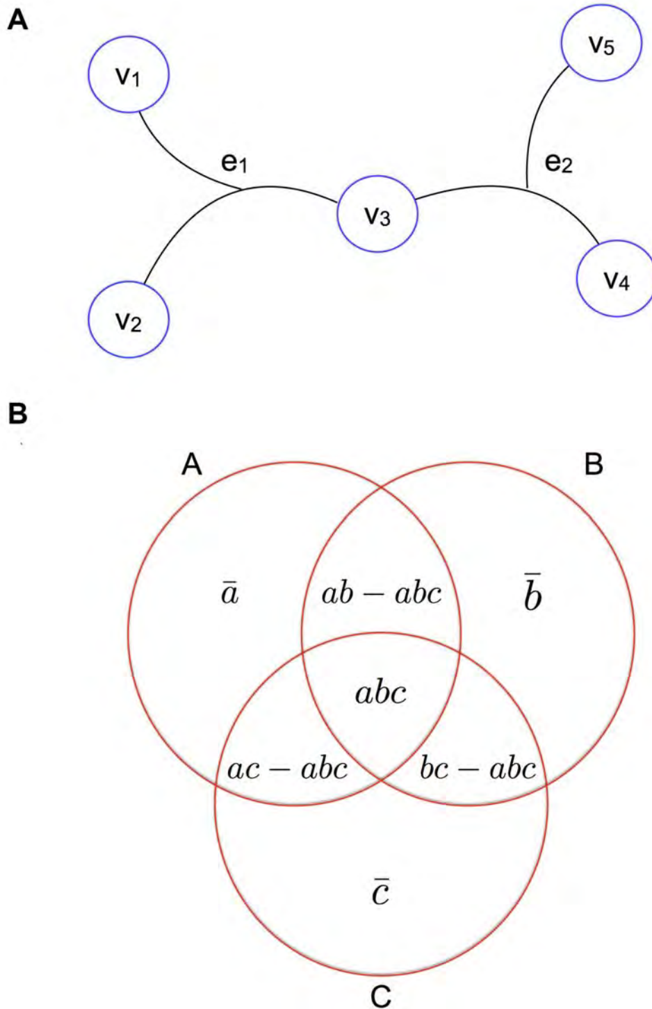
Fig 1. 3-way edges and intersections. (a) A small, 3-way network consisting of 5 nodes v_1, v_2, v_3, v_4 and v_5 and two 3-way edges e_1 and e_2 . Edge e_1 connects nodes v_1, v_2 and v_3 and edge e_2 connects nodes v_3, v_4 and v_5 . (b) Venn diagram for a 3-way intersection of species. a is the number of families present in species A, b is the number of families present in species B, c is the number of families present in species C, ab is the number of families present in species A and species B, ac is the number of families present in species A and species C, bc is the number of families present in species B and species C, abc is the number of families present in species A, B and C, \bar{a} is the number of families present only in species A, \bar{b} is the number of families present only in species B and \bar{c} is the number of families present only in species C.
